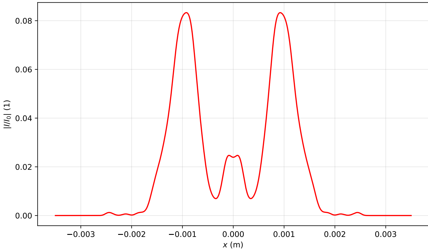
Intensity profile I(x, y = 0, z = 2.866)/I_0 , P_{in}=7.5P_{cr} , artificial time
